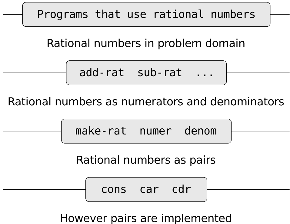
Figure 2.1: Data-abstraction barriers in the rational-number package.
