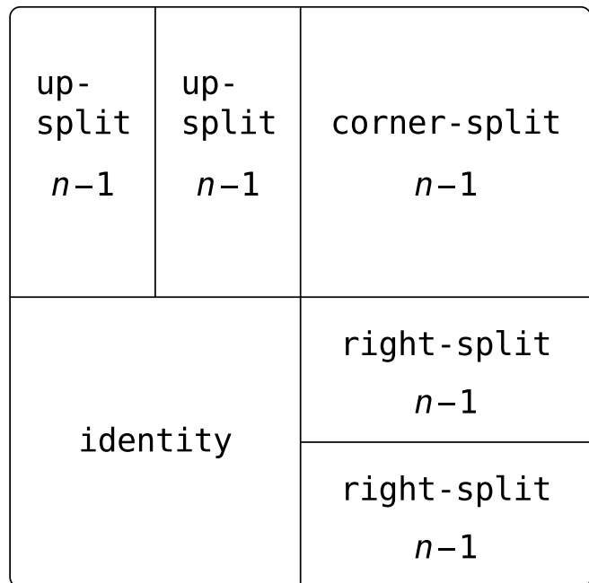
Figure 2.13: Recursive plans for right-split and corner-split.
