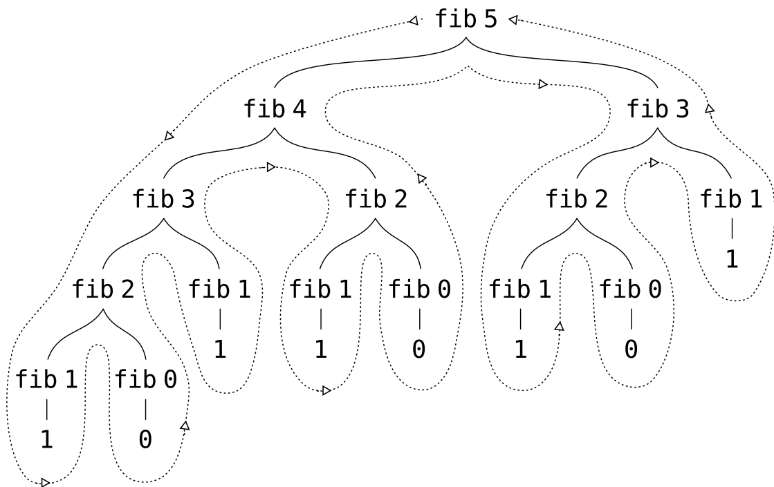
Figure 1.5: The tree-recursive process generated in computing (fib 5).
