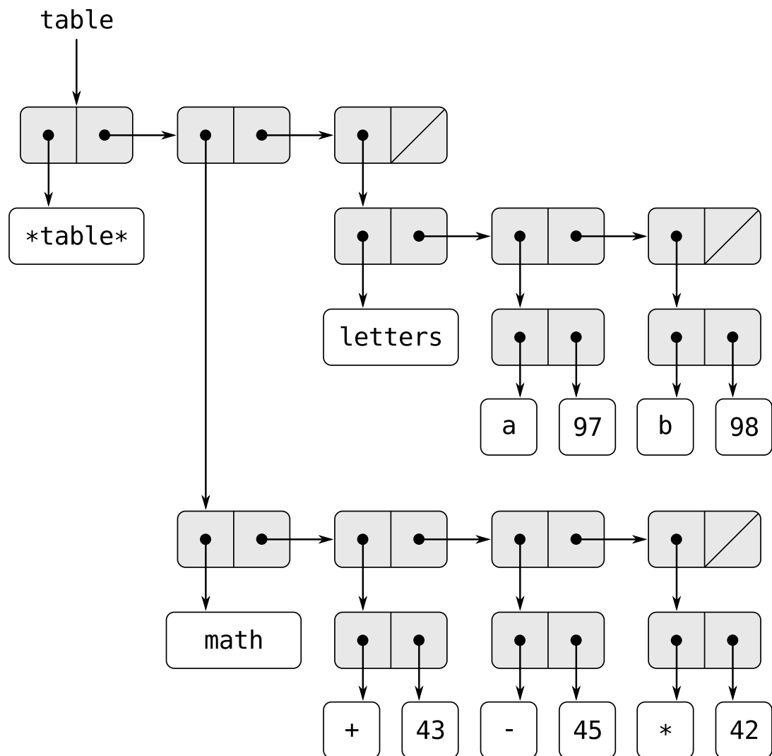
Figure 3.23: A two-dimensional table.
